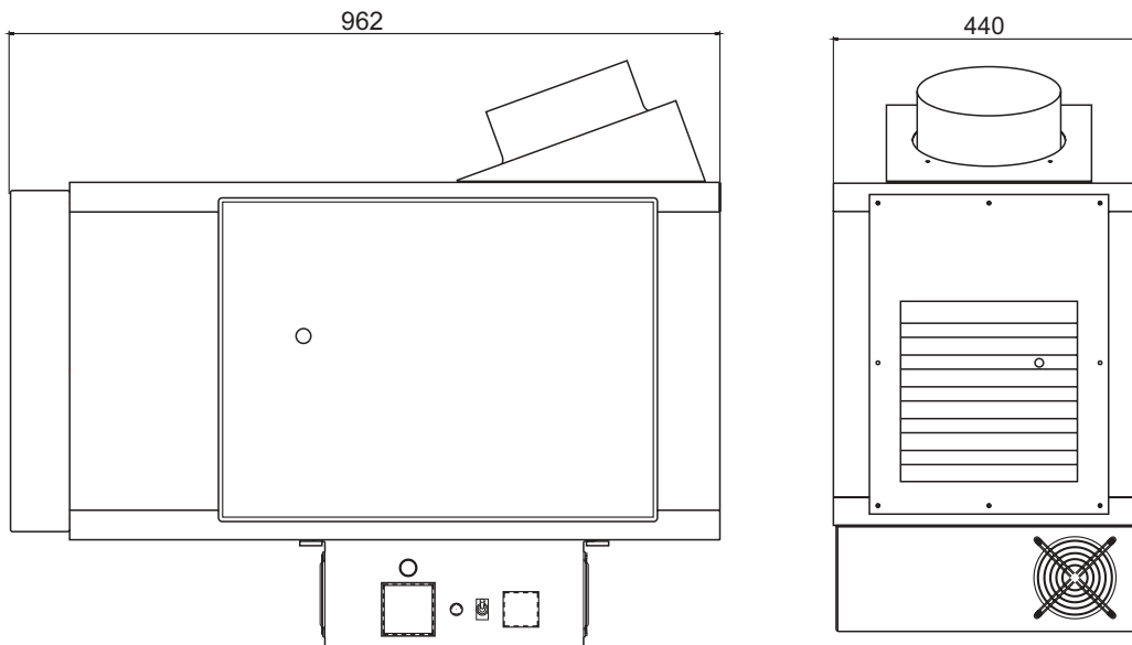
Special Lamp House for MP 75 E
